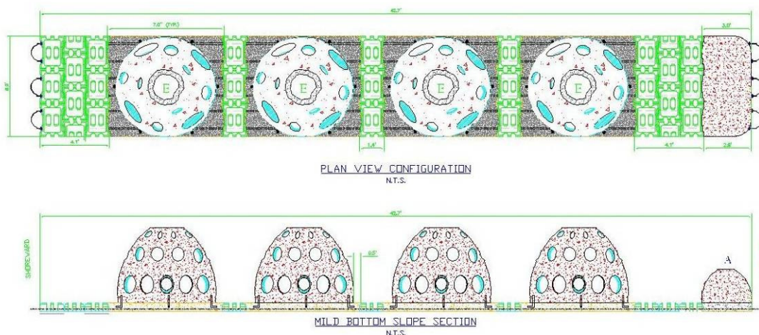
Figure 16. Reef Ball Units on Articulated Mat (HARRIS, Turk, & Mead, 2004))
